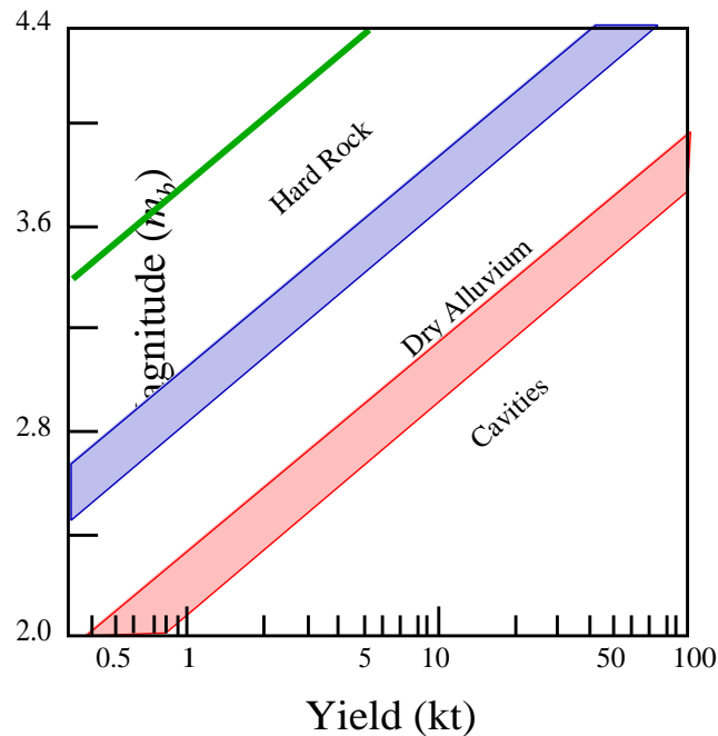
Figure 5: Estimate of expected teleseismic magnitude for a contained nuclear explosion as a function of yield. The effect of material on signal strength as well as decoupling is illustrated. After Hannon, 1985.
